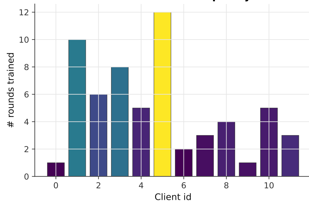
Client selection frequency
