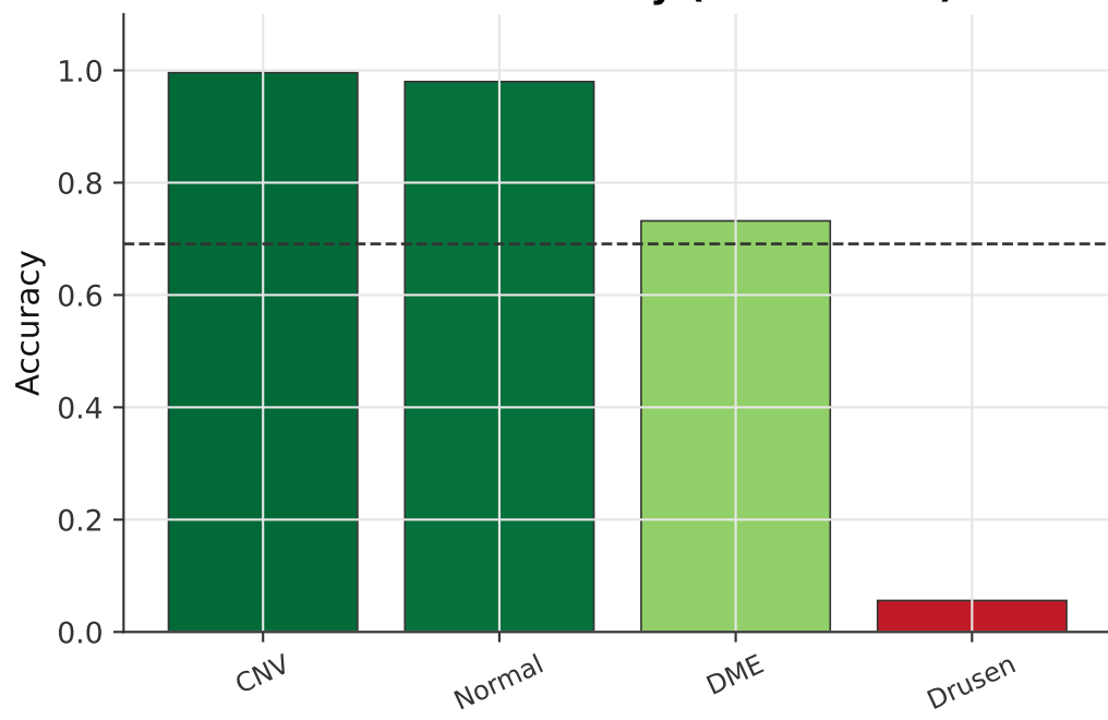
Per-class accuracy (final round)
