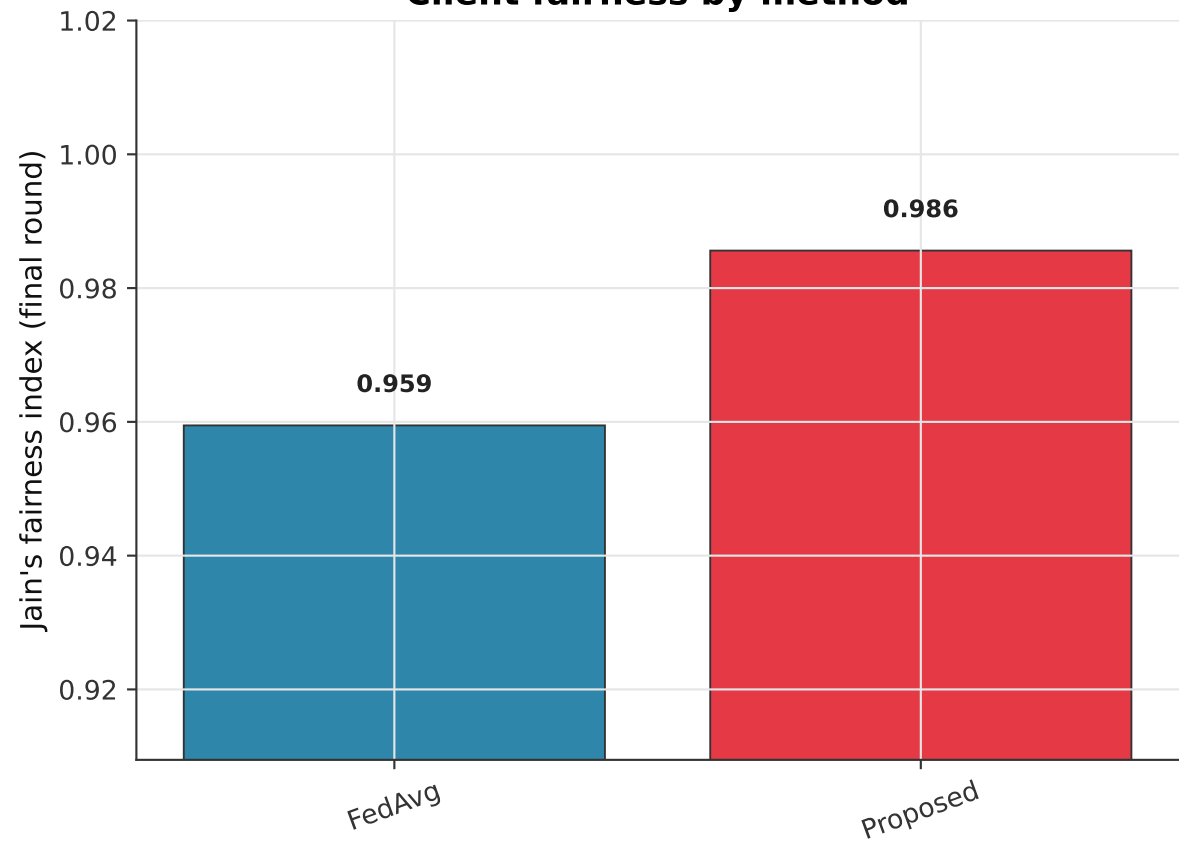
Client fairness by method
