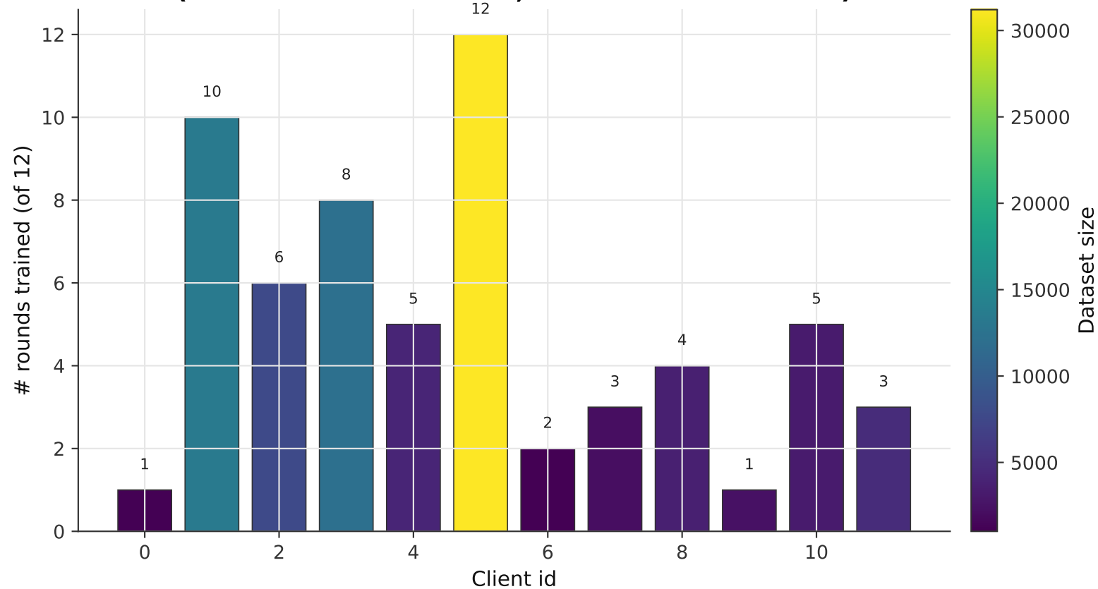
Client selection frequency — FedAvg (bar color = dataset size; taller = selected more)
