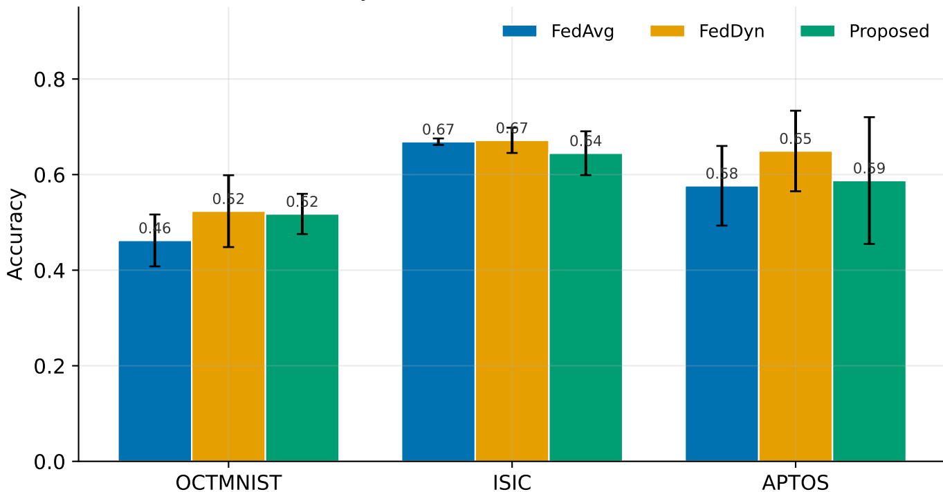
Accuracy across datasets — 40% label noise
