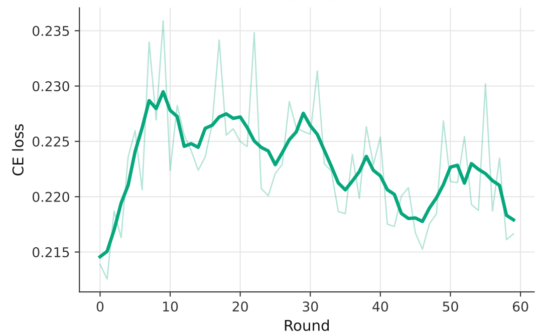
Test loss
