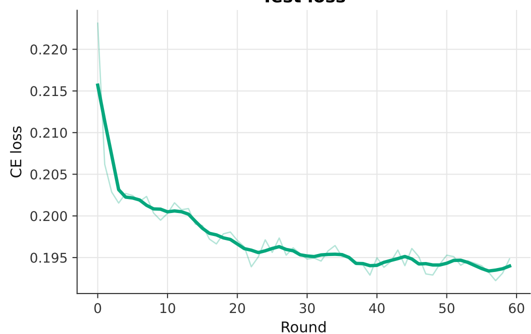
Test loss
