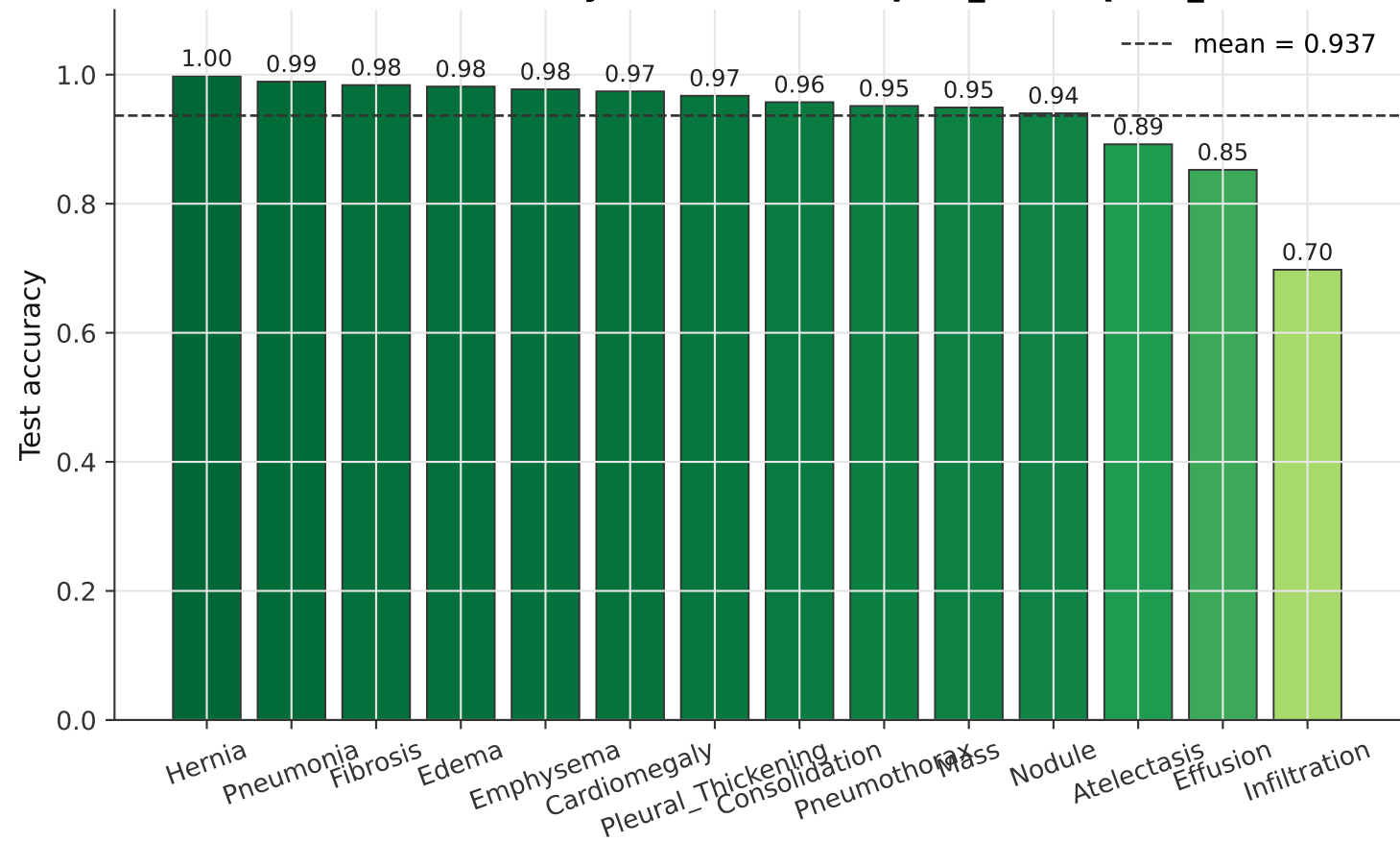
Per-class accuracy at round 59 — pow_d+shaped_wa
