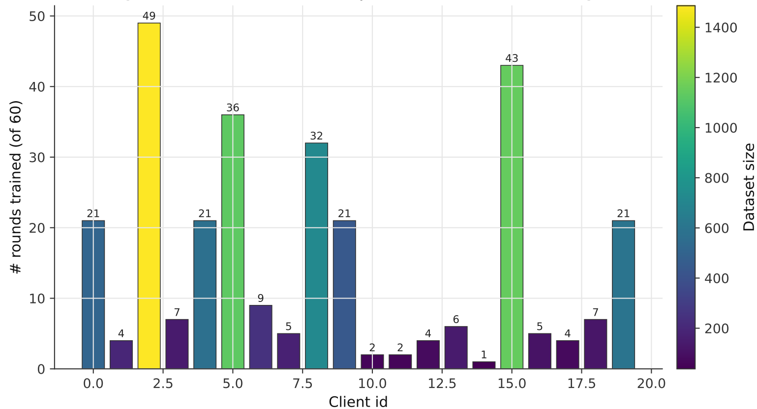
Client selection frequency — random+fedavg (bar color = dataset size; taller = selected more)
