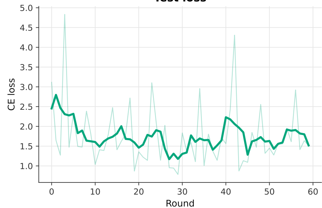
Test loss
