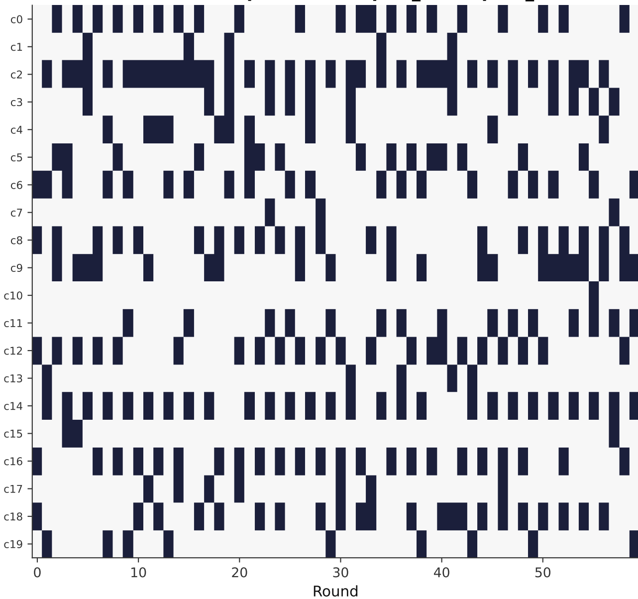
Active clients per round — pow_d+shapfed_wa
