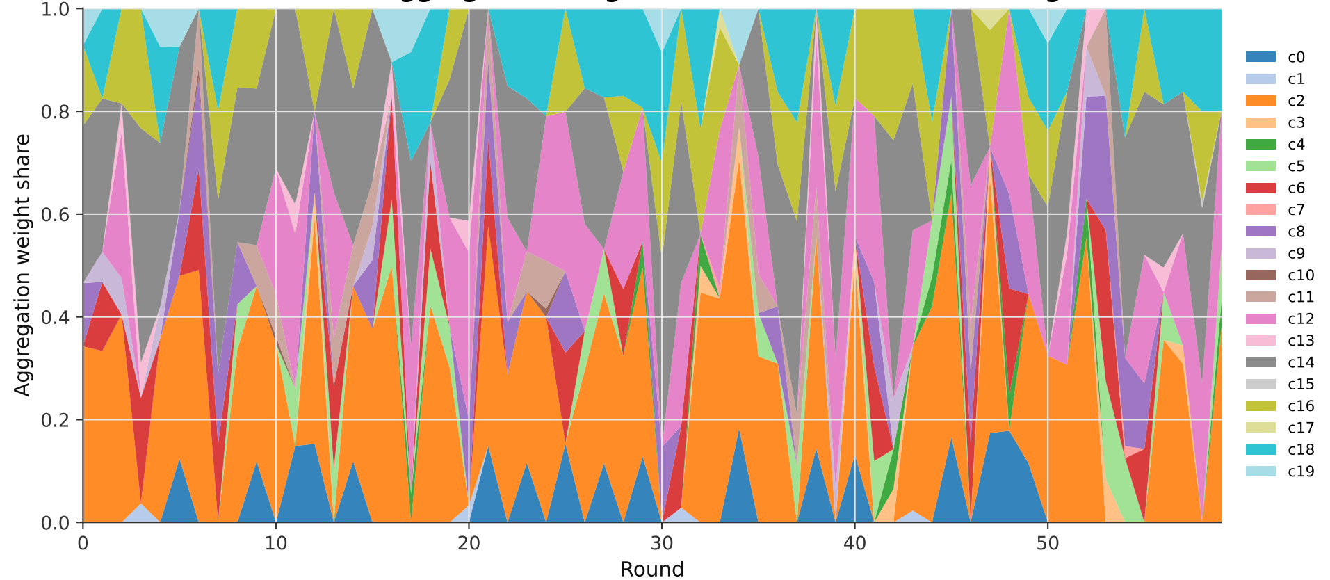
Per-client aggregation weights over time — random+fedavg
