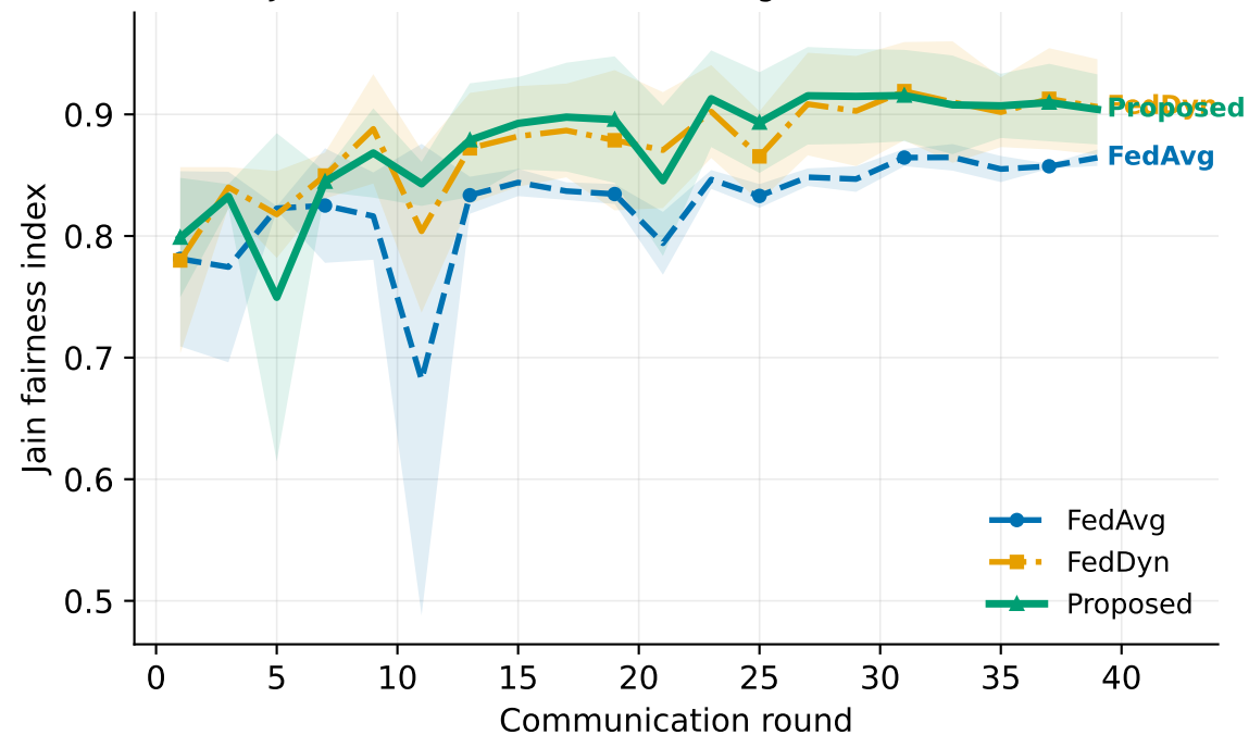
Jain fairness index over training — 40% label noise
