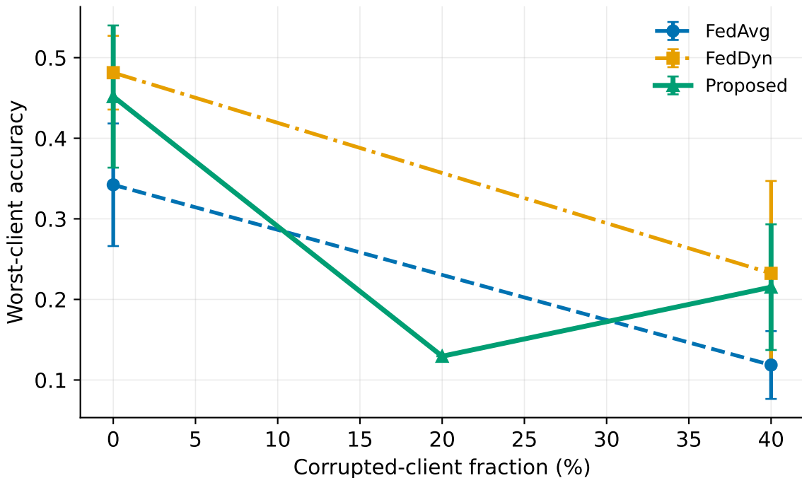
Worst-client accuracy vs. noise level — OCTMNIST
