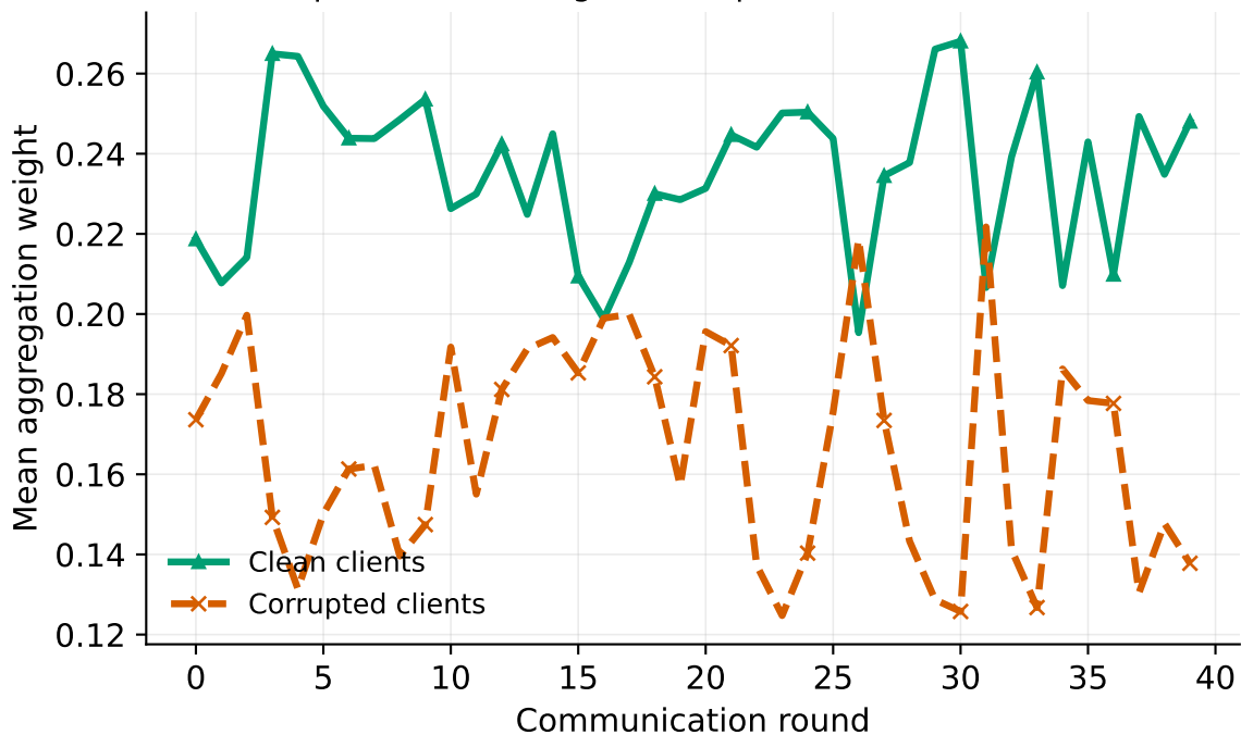
Proposed down-weights corrupted clients (40% noise)
