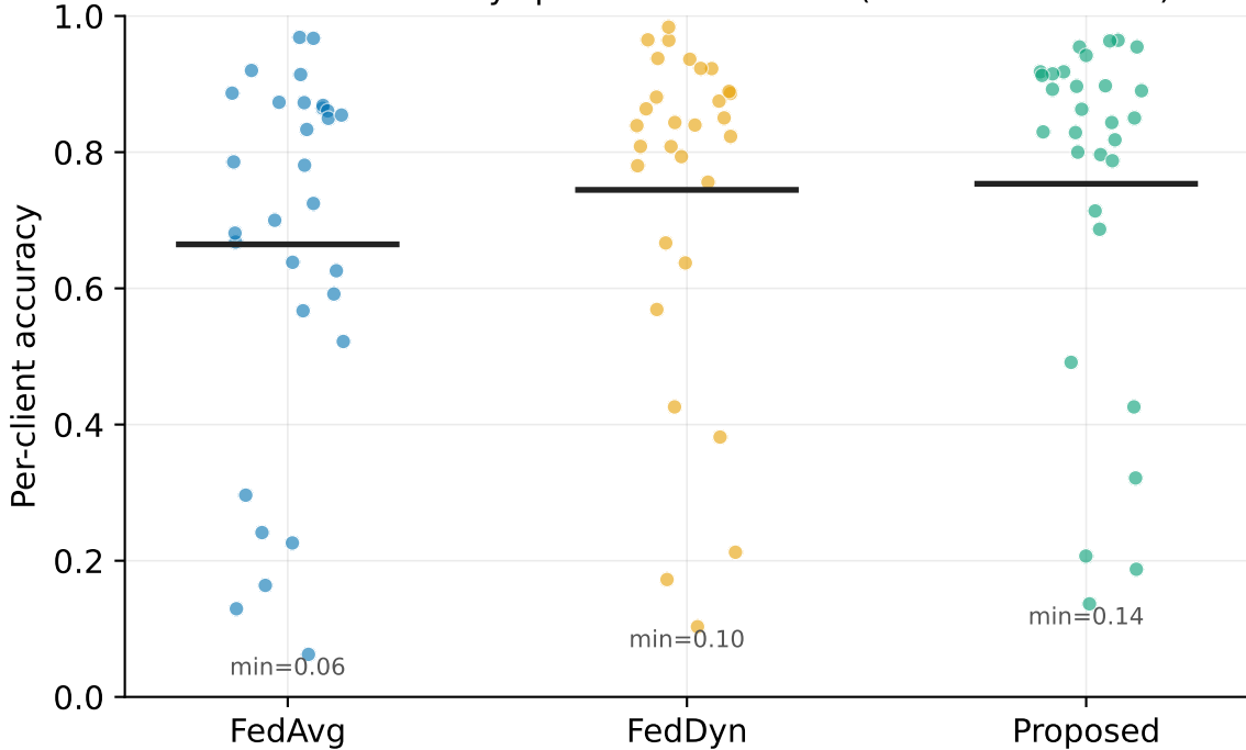
Per-client accuracy spread — 40% noise (black bar = mean)
