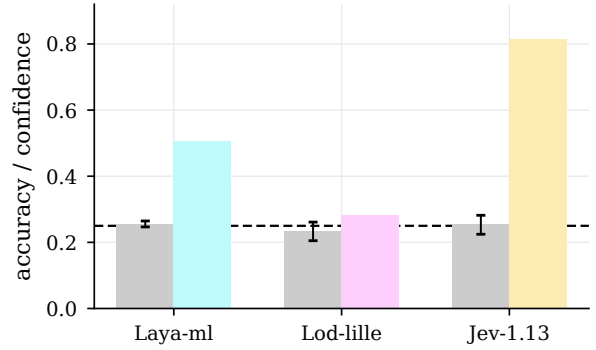
Figure 6: The semantics-free control. Per model, the ■ bar is accuracy (95% bootstrap CI) and the coloured bar is mean reported confidence (Laya-ml, Lod-lille, Jev-1.13); the dashed line is the four-option chance level. No option carries information, so the gap between the two bars is overconfidence: 0.250, 0.049 and 0.561. Jev-1.13’s condition is English.
