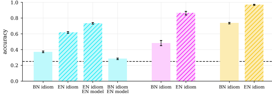
Figure 6: Accuracy by task language, grouped by model: ■ Laya-ml (four bars), ■ Lod-lille, ■ Jev-1.13. Solid bars are Bangla input, hatched bars English; Laya-ml’s third and fourth bars use the English-only checkpoint, the fourth being the control. Error bars 95% bootstrap CIs, dashed line chance. Every model gains between 23 and 38 points when the paired English entry is presented instead of the Bangla idiom.
