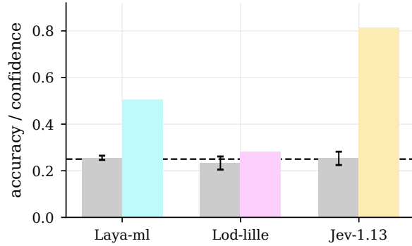
Figure 7: The semantics-free control. Per model, the ■ bar is accuracy (95% bootstrap CI) and the colored bar is mean reported confidence ( ■ Laya-ml, ■ Lod-lille, ■ Jev-1.13); the dashed line is the four-option chance level. No option carries information, so the gap between the two bars is overconfidence: 0.250, 0.049 and 0.561. Jev-1.13’s condition is English.
