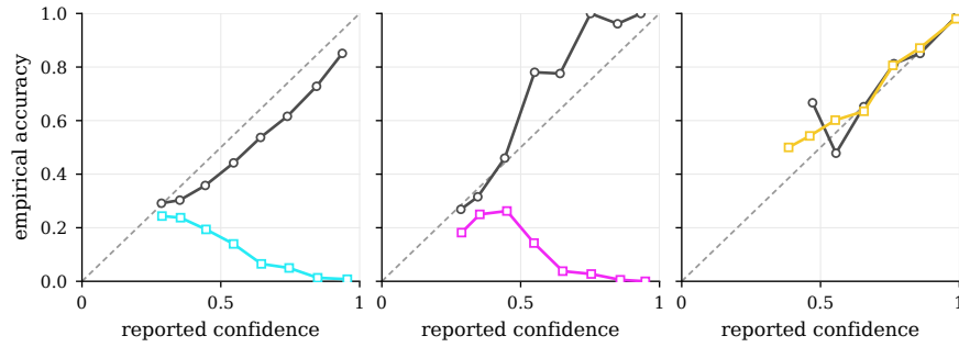
Figure 4: Reliability, 15 equal-width bins. Panels left to right: Laya-ml, Lod-lille, Jev-1.13. ■ circles are the random-distractor condition, squares in each panel’s own color the +literal one, and the gray dashed diagonal perfect calibration. Under D-LIT the two open models’ curves bend downward : the model is most wrong where it reports being most sure. Jev-1.13, in English, stays on the diagonal.
