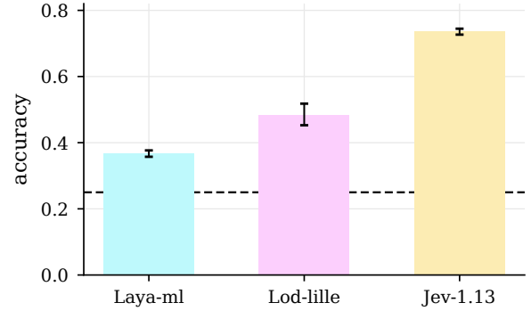
Figure 8: The matched three-way comparison. Bars left to right: ■ Laya-ml, ■ Lod-lille, ■ Jev-1.13. Black dashed line is chance, error bars 95% bootstrap CIs. This capability ordering is the baseline against which the calibration failures in §5.2–§5.3 should be read.
