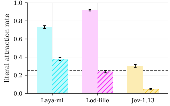
Figure 5: Literal attraction by model and task language, all six cells on the same 3,265 items (error bars 95% bootstrap CIs; dashed line the four-option chance level). ■ Laya-ml, ■ Lod-lille, ■ Jev-1.13; solid bars Bangla, hatched bars English. The Bangla ordering does not follow capability, and Jev-1.13’s English value matches the 0.047 of the English ladder. The cells are in Table 14 and their intervals in Appendix I.
