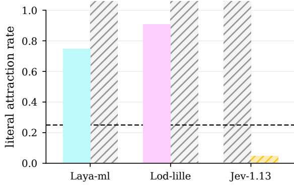
Figure 3: Literal attraction on the shared 3,265-item pool, by model and task language. Laya-ml, Lod-lille, Jev-1.13. Solid bars are Bangla; the hatched bar is Jev-1.13’s English condition, and the hatched blocks running past the top of the axis mark cells that were never run ; they are not values of 1.0. Jev-1.13’s low attraction cannot be read as a Bangla result; the experiment that would resolve the confound is exactly the two missing cells.
