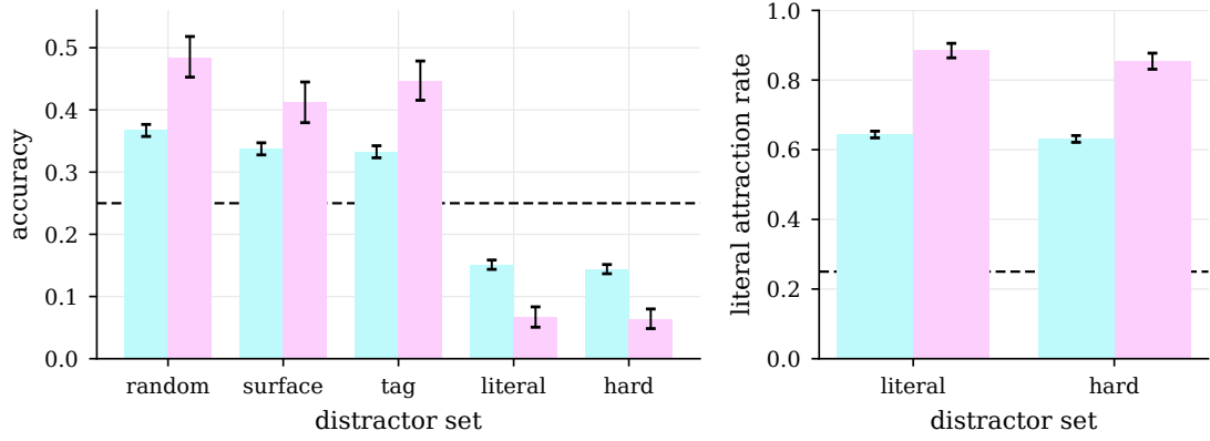
Figure 8: The distractor ladder (left) and literal attraction rate (right) for the two open arms. ■ Laya-ml ( n = 8,876 ), ■ Lod-lille ( n = 888 ); black dashed line is chance (0.250), error bars 95% bootstrap CIs. Surface- and tag-matched distractors cost a few points. Inserting the idiom’s own literal gloss (D-LIT) collapses both models far below chance, and collapses the stronger model harder: Lod-lille leads Laya-ml by +0.133 on random distractors and trails it by -0.070 once the literal gloss is present. On the right, both models prefer the literal reading to the figurative one on the majority of items.
