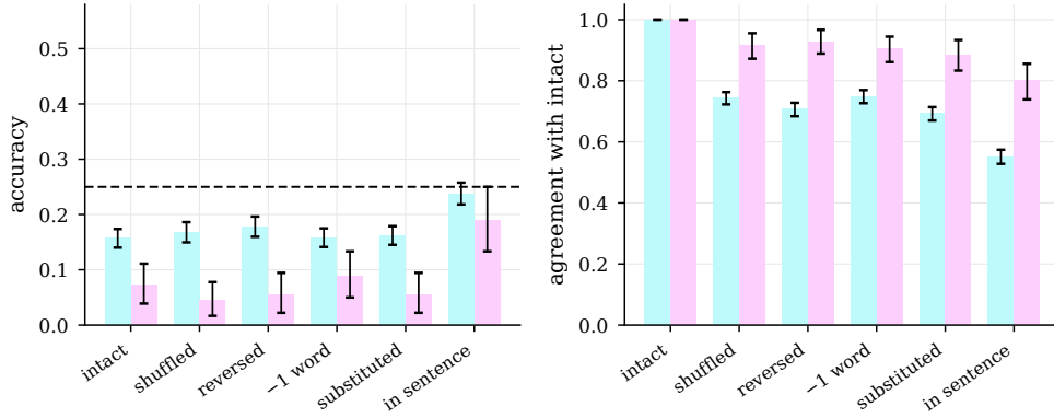
Figure 9: Unit integrity: the idiom is perturbed, the options held fixed. ■ Laya-ml, ■ Lod-lille; error bars 95% bootstrap CIs, dashed line chance (left panel). Left : accuracy. Right : agreement with the answer on the intact idiom. Scrambling and reversing a non-compositional expression does not meaningfully hurt either model, which is the bag-of-words signature.
