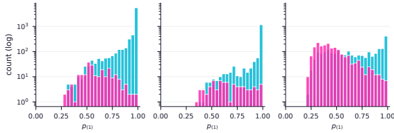
Figure 8: Top-1 probability by outcome, log count; left to right, MathQA-style, CompMath-MCQ and HARP. ■ correct, ■ incorrect. On the easier benchmarks errors sit in the middle of the range and vanish at the top. On HARP the correct and incorrect distributions overlap heavily, which is the distributional form of the deferral collapse in §5.4.
