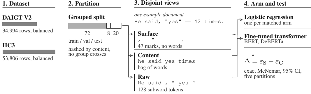
Fig. 1. The measurement pipeline. Stage 3 puts one constructed document through each view and shows what survives. The transformer is a reference point, not a third arm.
