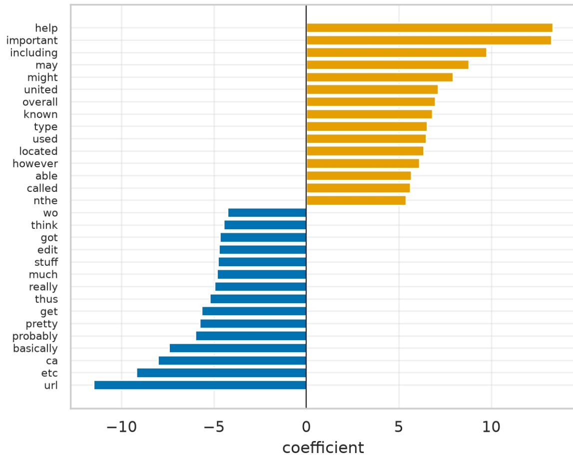
HC3: LogReg [liblinear] coefficients (left = human, right = machine)
