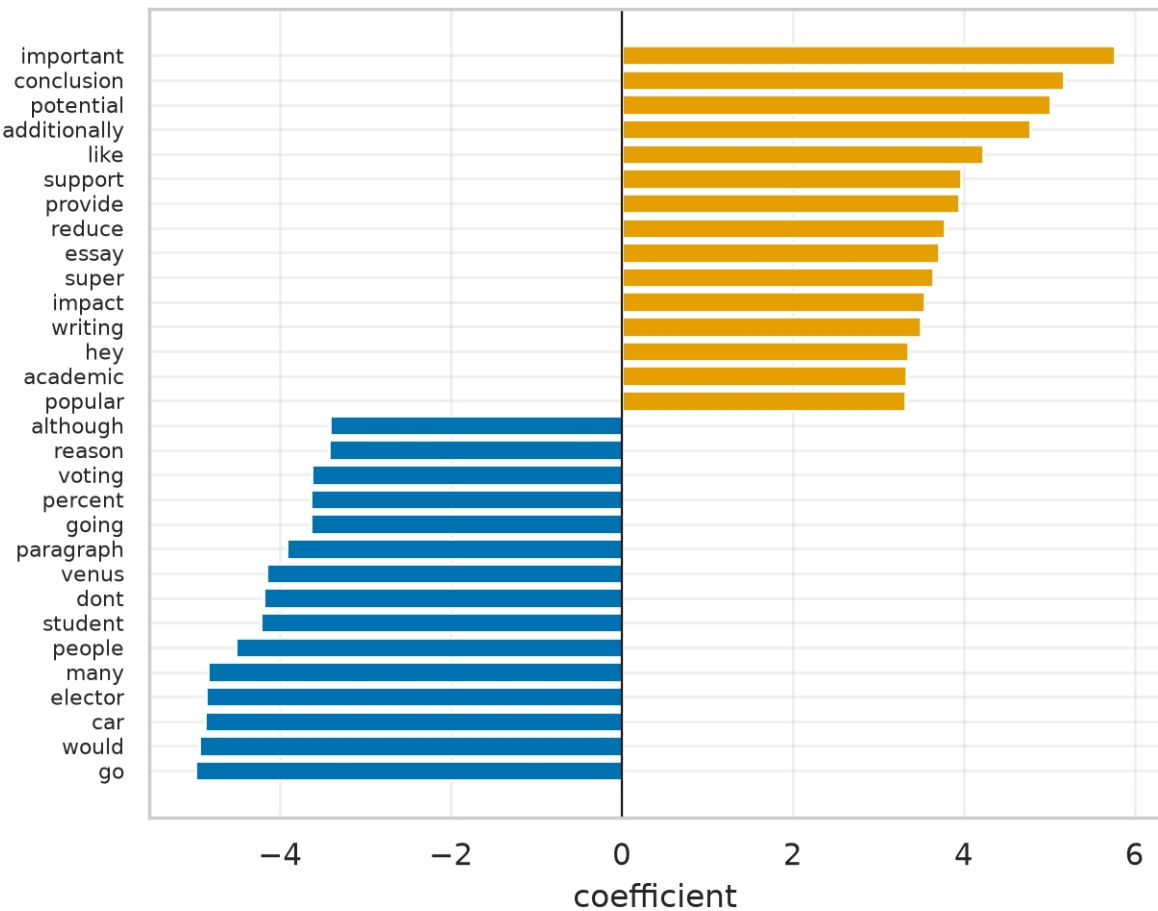
DAIGT V2: LogReg [liblinear] coefficients (left = human, right = machine)
