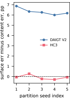
(c) Five group-aware partitions
