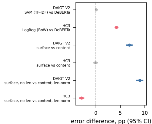
(f) Paired intervals
