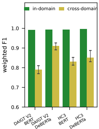
(e) Cross-dataset transfer, 3 seeds
