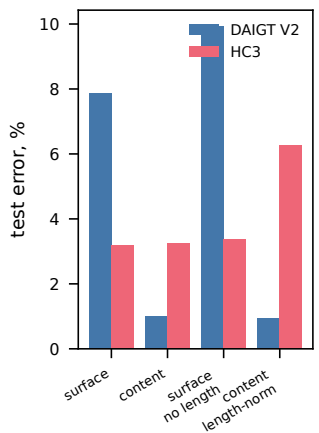
(e) Cross-dataset transfer, 3 seeds
