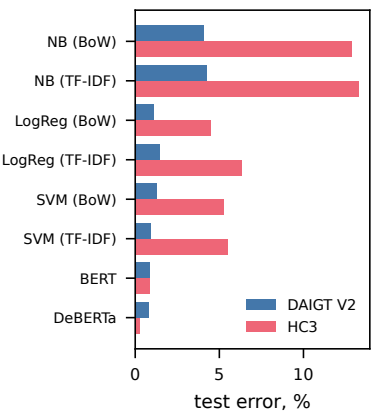
(a) All eight configurations
