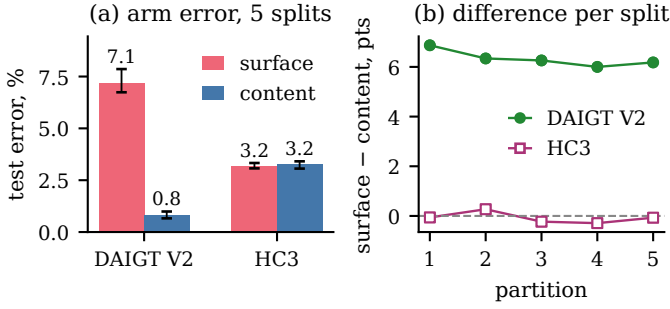
Fig. 2. Arm error and the per-split difference. Filled marks a significant surface-vs-content difference ( p < 0.05 ).
