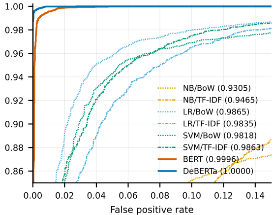
(b) HC3, detail
