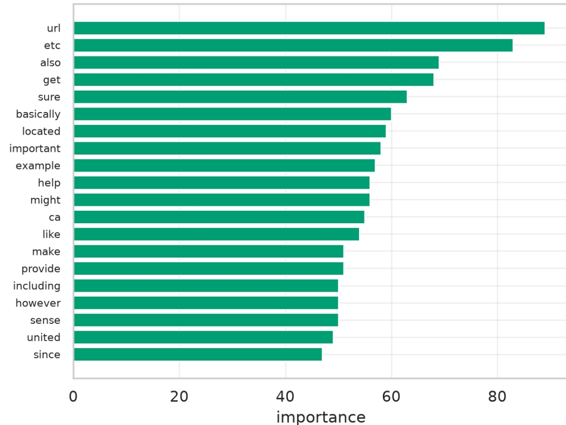
HC3: LightGBM gain importance
