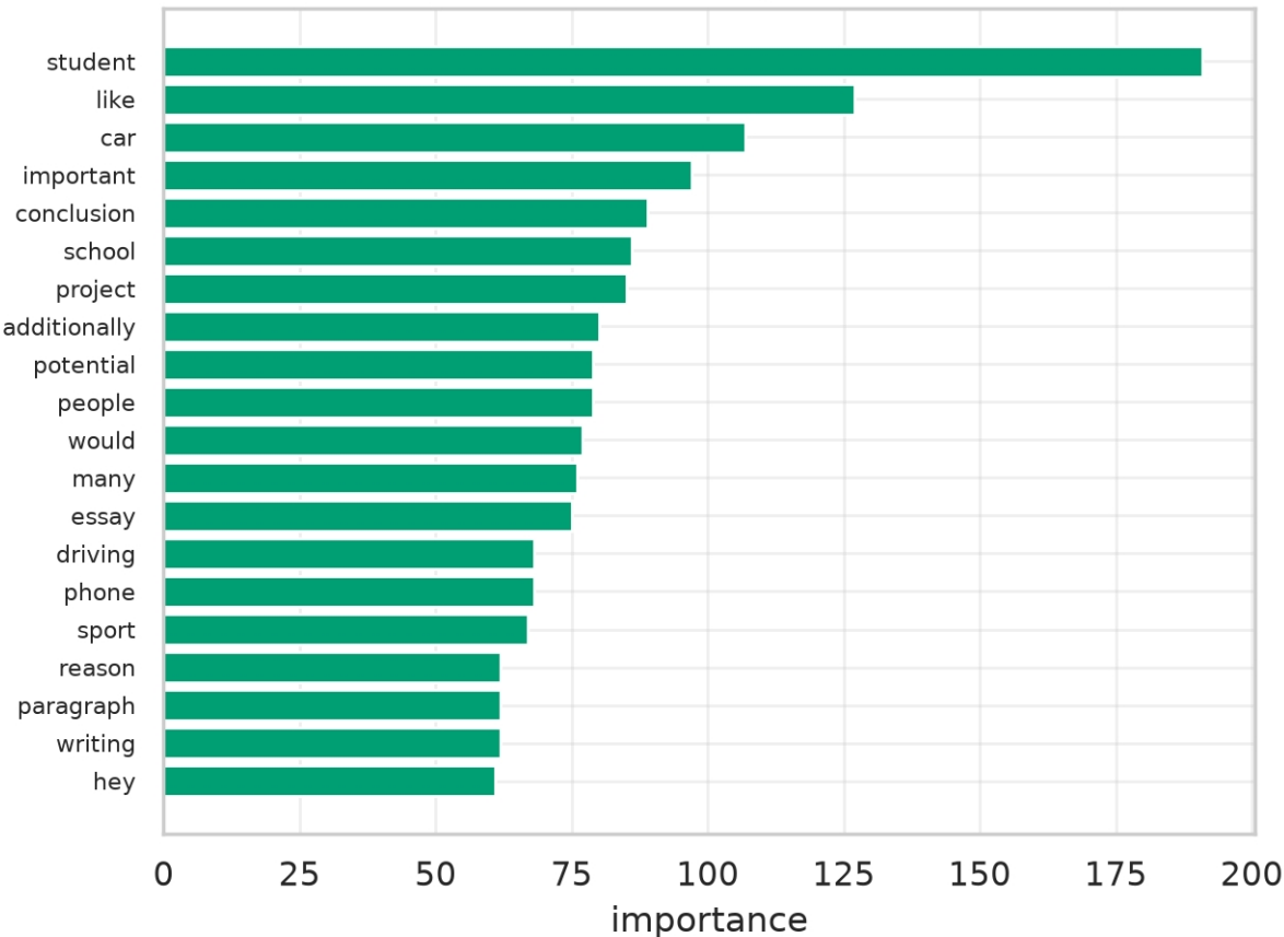
DAIGT V2: LightGBM gain importance
