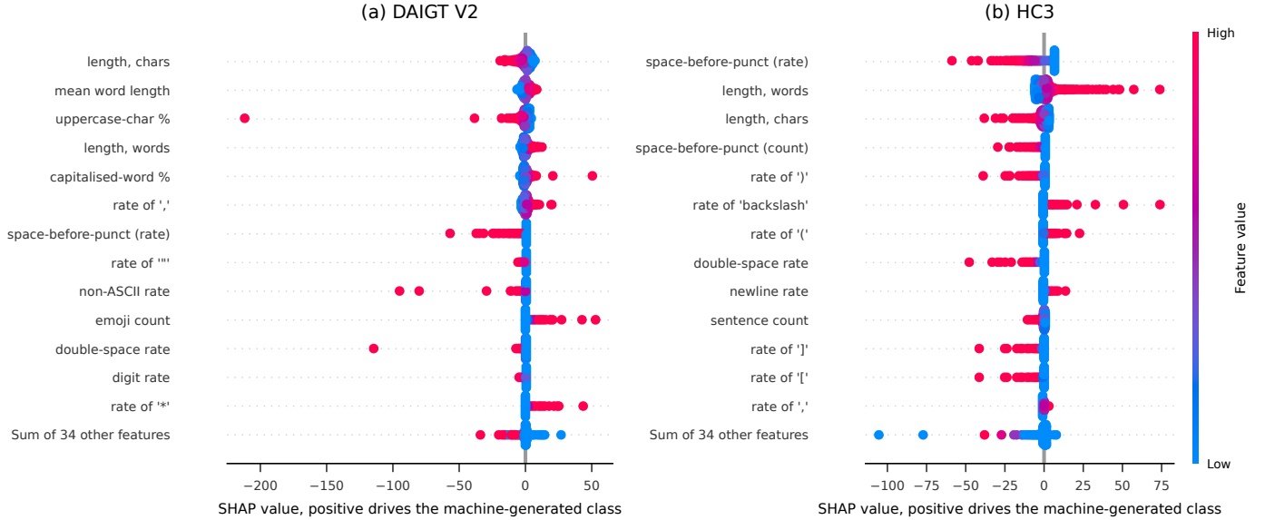
Fig. 4. SHAP attributions over the surface-only arm, computed exactly with a linear explainer on 2,000 held-out documents per corpus. Each point is one document, positioned by its contribution to the machine-generated class and coloured by feature value.
