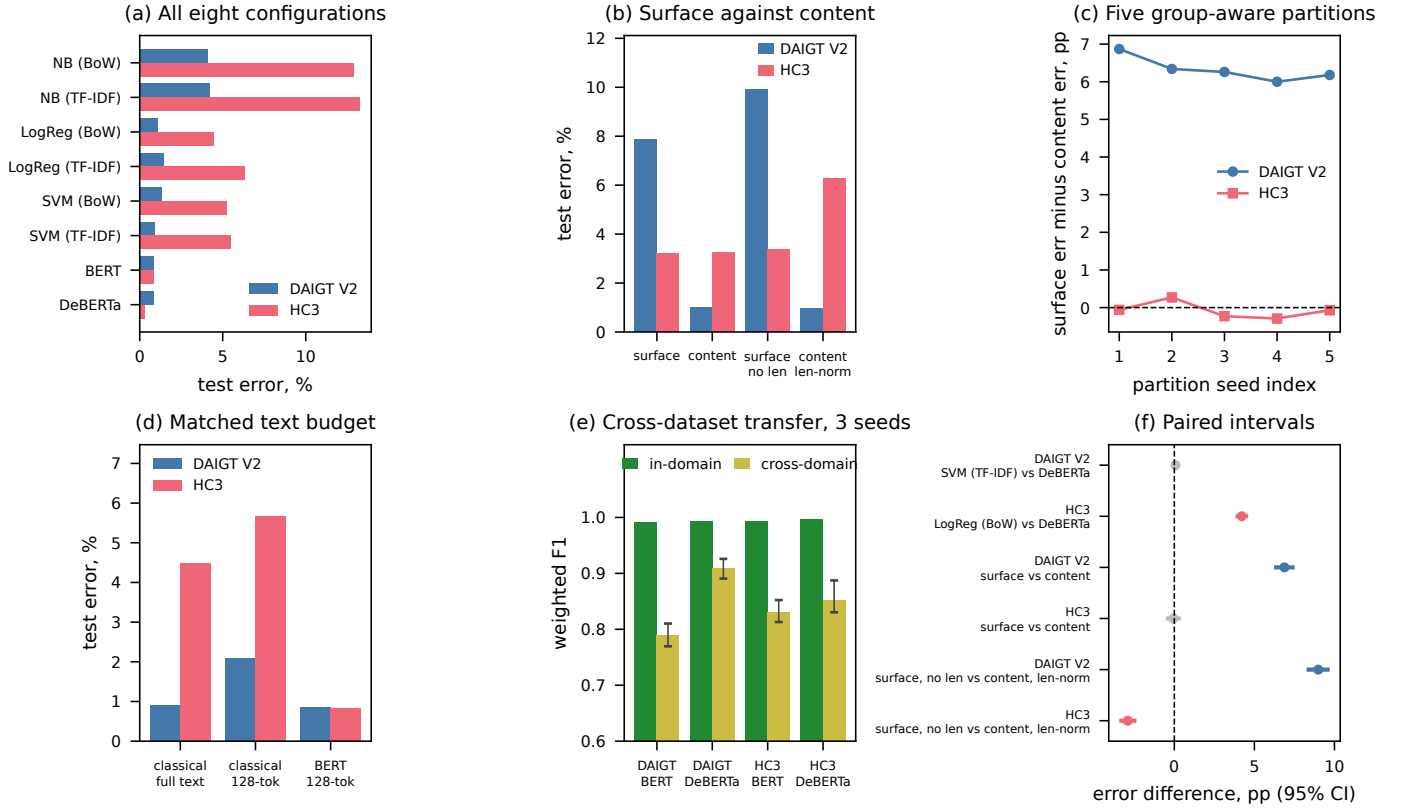
Fig. 5. Every headline result in one view. Panels give the model ranking (a), the decomposition with and without the length channel (b), the surface-minus-content difference across five partitions (c), the matched text budget (d), cross-corpus transfer (e), and the paired intervals behind each significance claim (f), where grey marks an interval containing zero.
