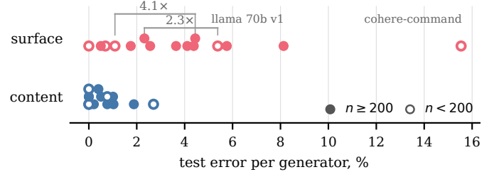
Fig. 2. Test error per DAIGT V2 generator. Brackets join same-model pairs from different contributors.
