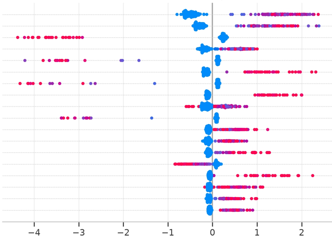
HC3: SHAP value distribution (LightGBM)
