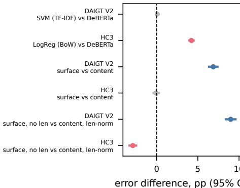
(f) Paired intervals
