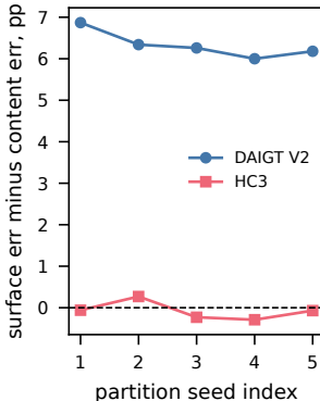
(f) Paired intervals
