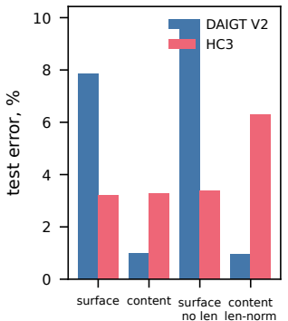
(b) Surface against content
