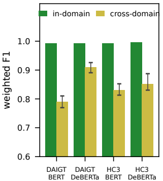
(e) Cross-dataset transfer, 3 seeds
