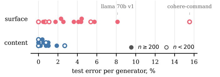
Fig. 2. Test error per DAIGT V2 generator, one point each, surface against content.
