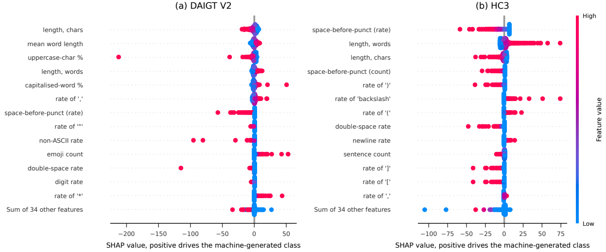
Fig. 5. Shapley attributions for the surface arm, the twelve highest-magnitude features per corpus with the remaining thirty-four summed. Colour is the feature value. HC3 is led by one cue; DAIGT V2 is led by size.
