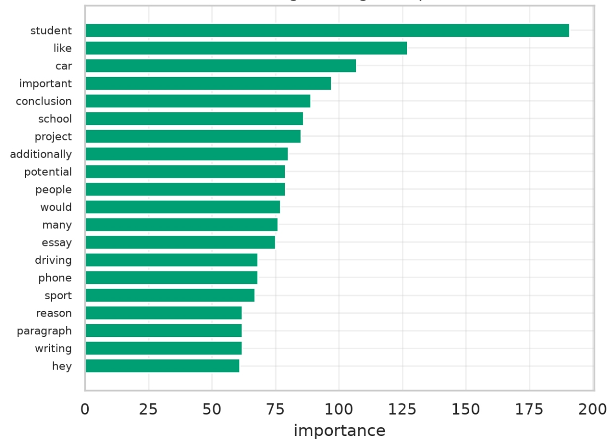
DAIGT V2: LightGBM gain importance
