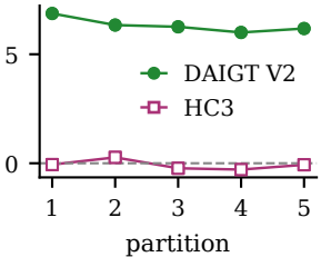
(b) difference per split
