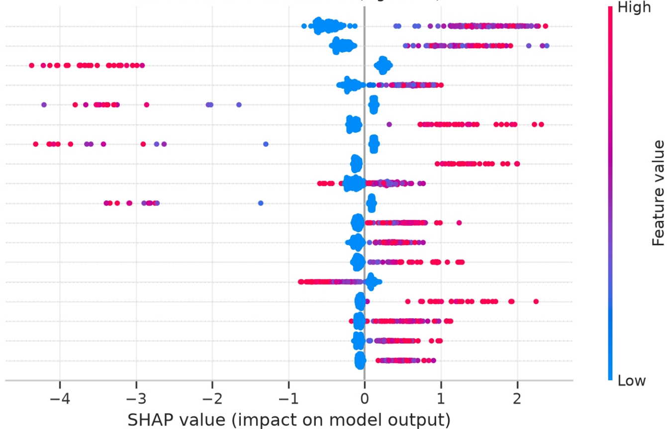
HC3: SHAP value distribution (LightGBM)
