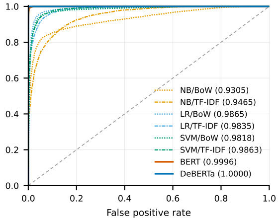
(b) HC3
