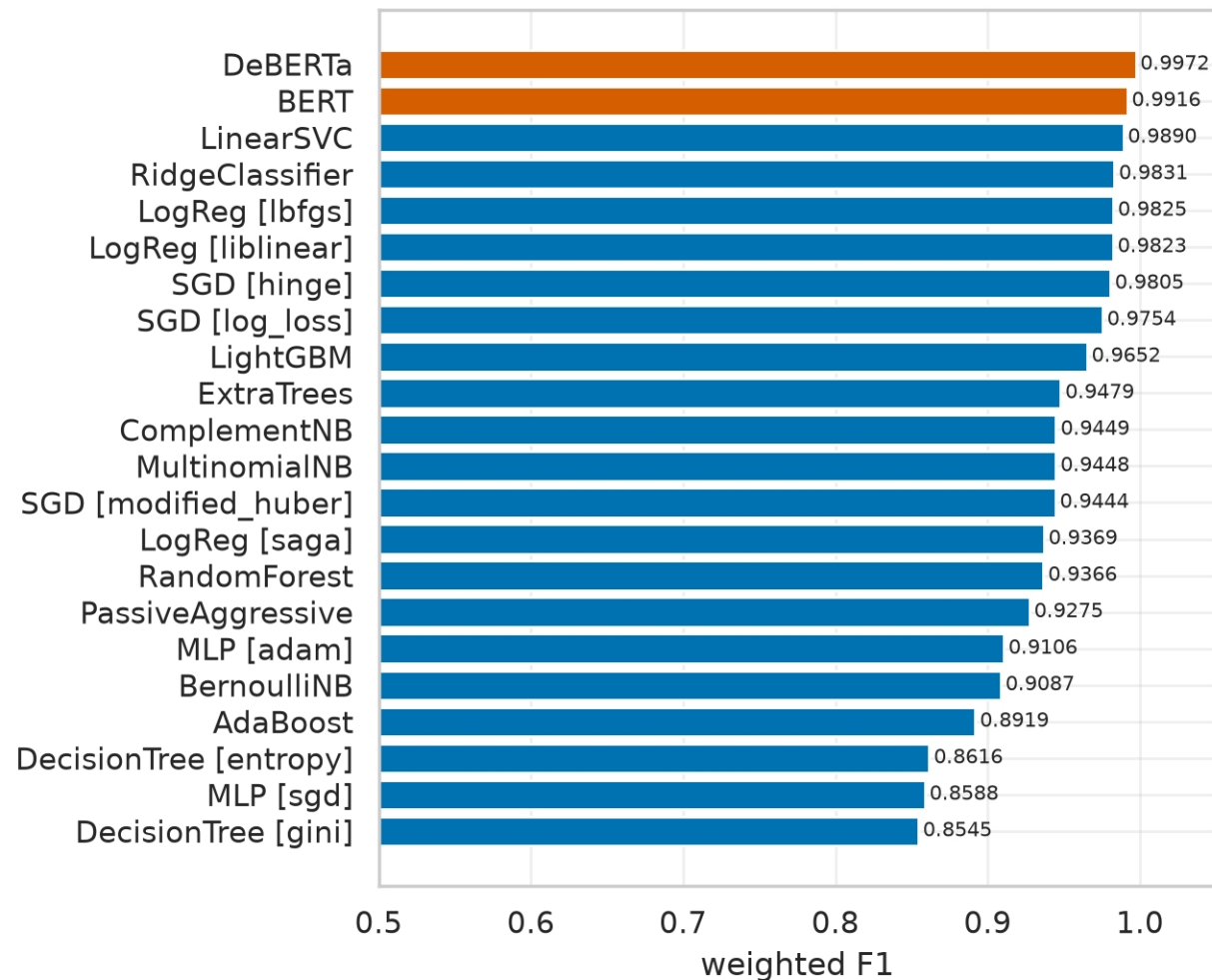
HC3
