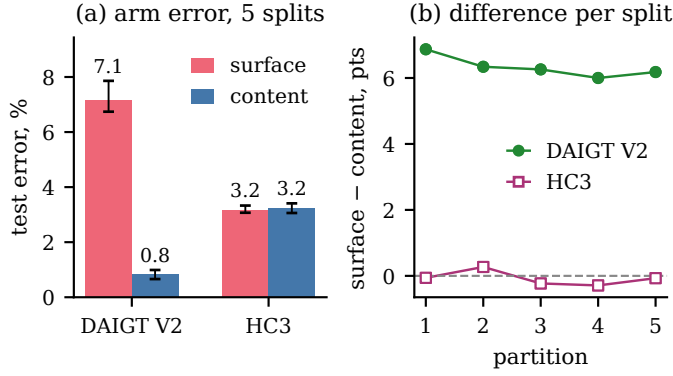
Fig. 2. Arm error and the per-split difference. Filled marks p < 0.05 .
