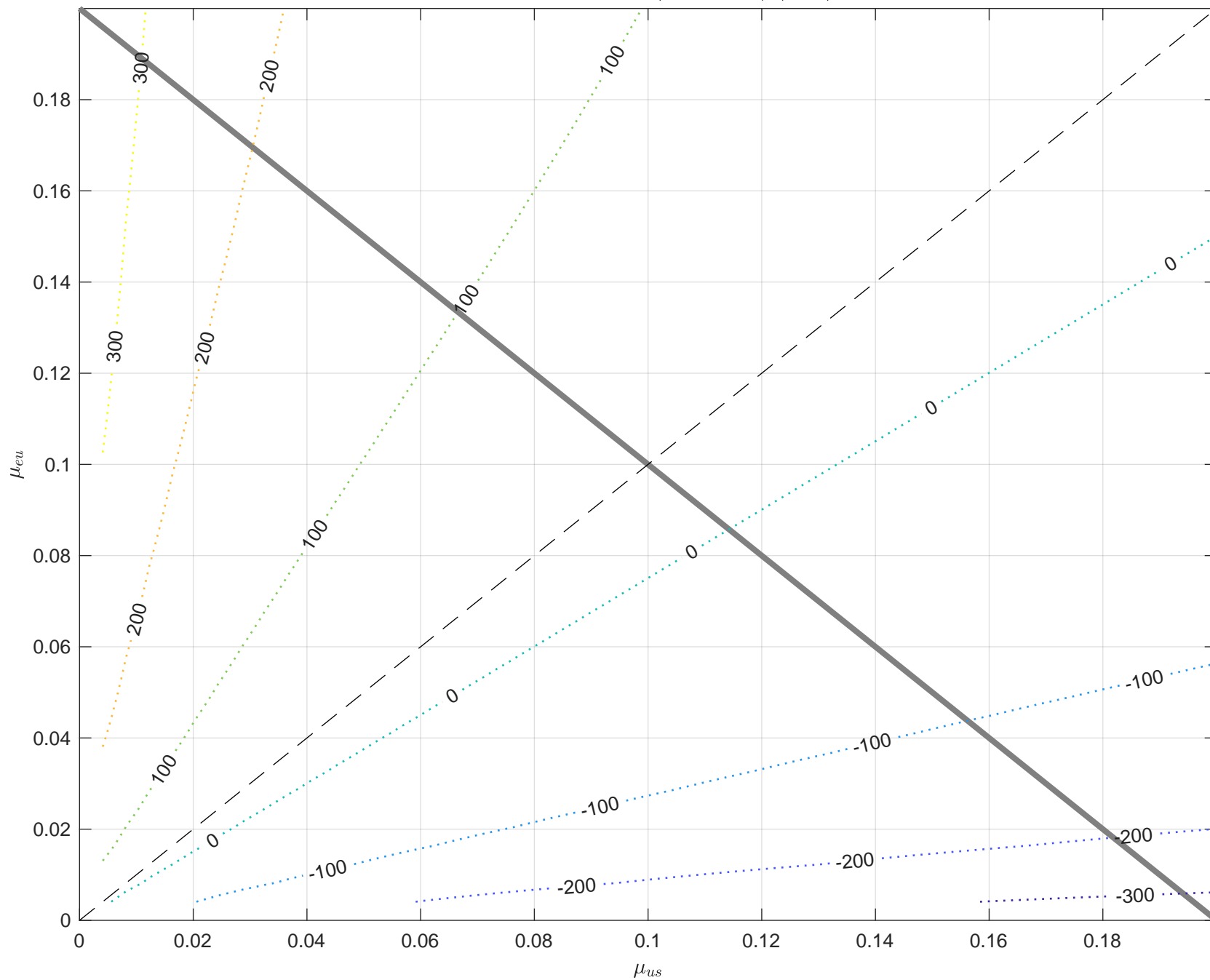
Iso-Dollar Premium ( R^m - R^{*,m} ) (BPS)
