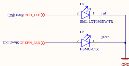
Indicator LED
