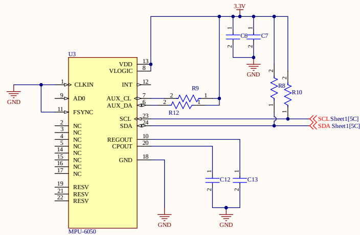
Accelerometer
