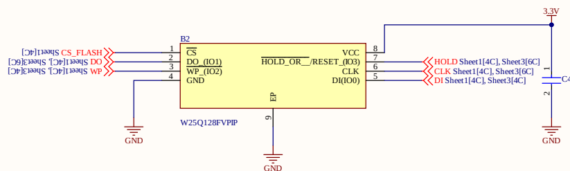
Flash Memory
