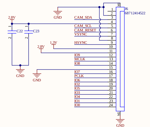
Camera
