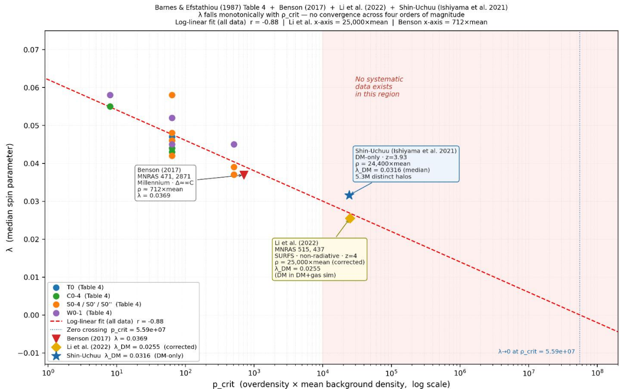
Figure 4 (revised). Halo spin parameter \lambda vs overdensity threshold \rho_{\text{crit}} . Barnes & Efstathiou (1987). Benson (2017), Li et al. (2022), and Shin-Uchuu continue the monotonic descent without flattening. Li et al. x-axis = 25,000 \times \text{mean} at z=0 , derived from \Delta_{200} mean density definition at z=4 . Dashed extrapolation projects to \lambda \rightarrow 0 at \rho_{\text{crit}} \sim 10^7 – 10^8 . No free parameters in the placement of the modern points. This is the empirical measurement of E[\lambda] \rightarrow 0 predicted by A.4–A.6.
