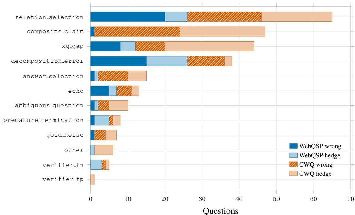
Figure 8.1: The failure histogram of Table 8.2 drawn as stacked bars, ordered by total. Wrong and hedge are shown as separate segments and are never pooled, because they describe different failure semantics. The asymmetry the section below analyses is visible as the length of the CWQ segments on composite_claim and kg_gap against their near-absence on WebQSP. Generated from results/phase4/thesis_numbers.json.
