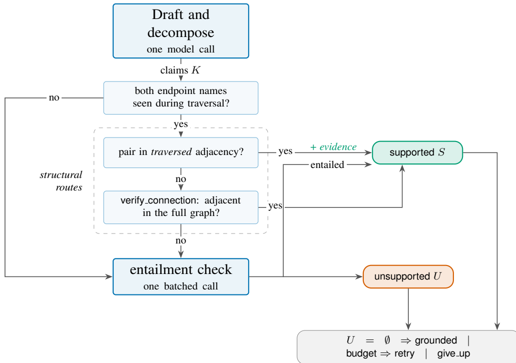
Figure 5.1: The path of a single atomic claim through the layer, mirroring Algorithm 2. Three tests are tried in a fixed order and a claim leaves at the first one that settles it. The two structural routes are boxed. Only the first of them adds to the supporting-triple list. That asymmetry is why Section 5.6 can report evidence for some grounded answers and not others. A claim naming an entity the agent never traversed skips both structural routes entirely, since the name-to-identifier map is built from traversed triples alone.
