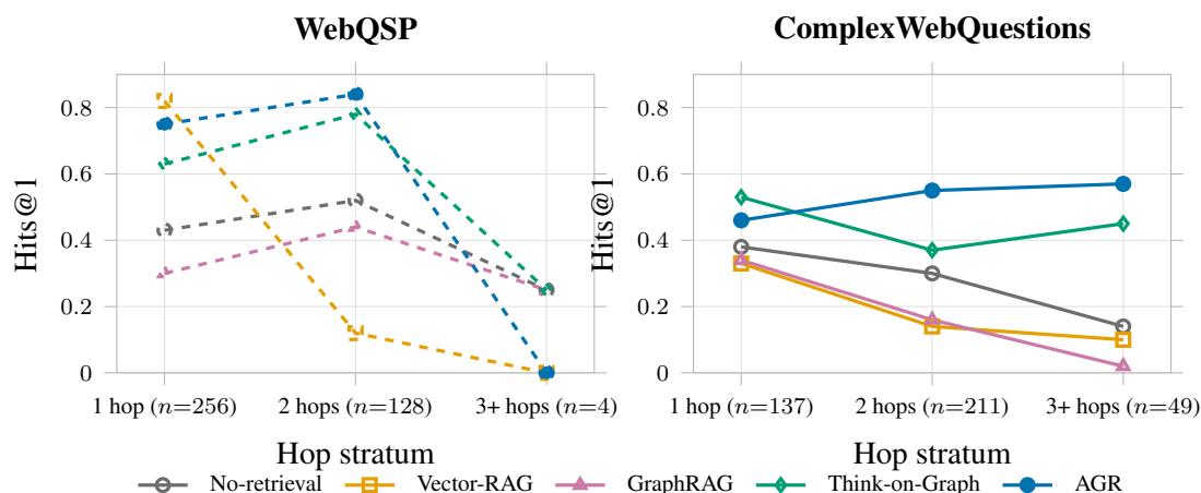
Figure 7.1: Hits@1 across hop strata. The shape is the finding: on ComplexWebQuestions AGR is the only system whose accuracy rises with hop count. Every other profile ends below where it started — three of them monotonically, Think-on-Graph by falling and partly recovering. WebQSP is drawn dashed because its h3plus stratum holds four questions and cannot carry a trend. The stratum sizes are printed on the axis for that reason. The unreachable stratum is omitted here and discussed below, since by construction it measures assertion rather than accuracy. Generated from results/phase4/thesis_numbers.json.
