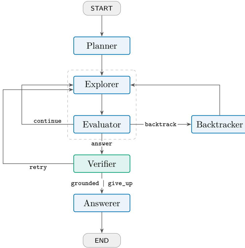
Figure 1: The AGR state machine. The dashed region is the Explorer \leftrightarrow Evaluator search loop; Evaluator \rightarrow Backtracker \rightarrow Explorer restores an earlier frontier; Verifier \rightarrow Explorer is verification-driven re-exploration. All three cycles are bounded by the budgets of Section 3.3. Every path from Evaluator to Answerer passes through the Verifier.
