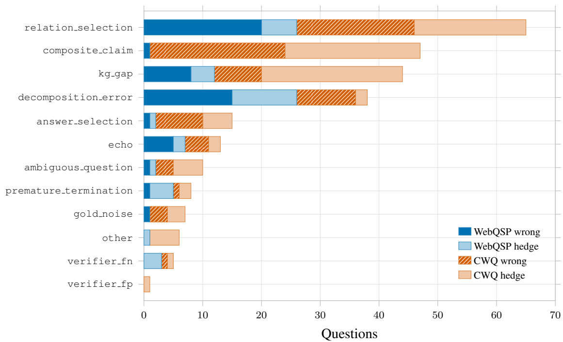
Figure 5.3: The failure histogram of Table 5.14 drawn as stacked bars, ordered by total. Wrong and hedge are shown as separate segments and are never pooled, because they describe different failure semantics. The asymmetry the section below analyses is visible as the length of the CWQ segments on composite.claim and kg.gap against their near-absence on WebQSP. Generated from results/phase4/thesis_numbers.json .
