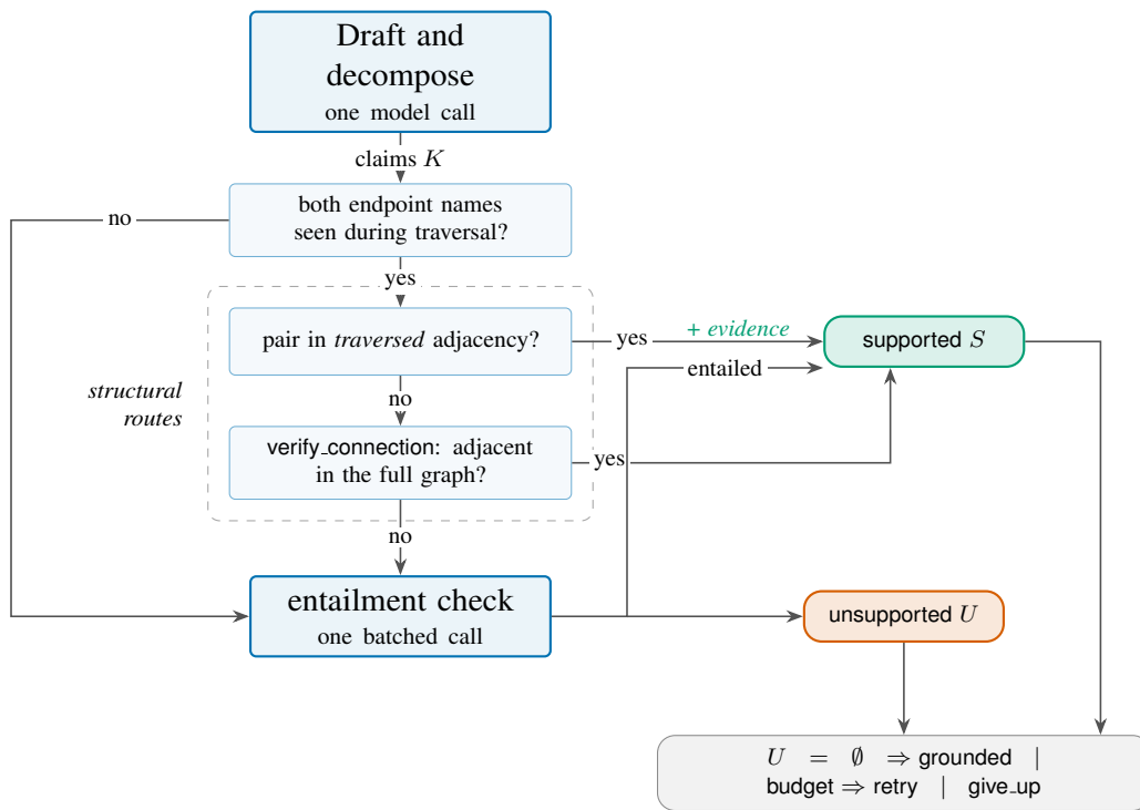
Figure 4.2: The path of a single atomic claim through the layer, mirroring Algorithm 2. Three tests are tried in a fixed order and a claim leaves at the first one that settles it. The two structural routes are boxed. Only the first of them adds to the supporting-triple list. That asymmetry is why Section 4.18 can report evidence for some grounded answers and not others. A claim naming an entity the agent never traversed skips both structural routes entirely, since the name-to-identifier map is built from traversed triples alone.
