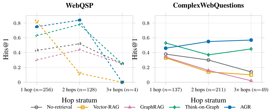
Figure 8.1: Hits@1 across hop strata. The shape is the finding: on ComplexWebQuestions AGR is the only system whose accuracy rises with hop count. Every other profile ends below where it started — three of them monotonically, Think-on-Graph by falling and partly recovering. WebQSP is drawn dashed because its h3plus stratum holds four questions and cannot carry a trend. The stratum sizes are printed on the axis for that reason. The unreachable stratum is omitted here and discussed below, since by construction it measures assertion rather than accuracy. Generated from results/phase4/thesis_numbers.json.
