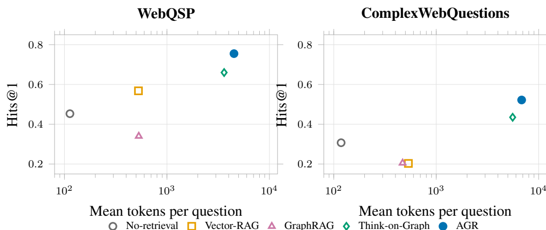
Figure 6.2: Accuracy against token cost, one point per system. The horizontal axis is logarithmic: the agentic systems cost roughly an order of magnitude more than the one-shot ones, and a linear axis would compress every non-agentic system into a single column. Read this figure for the token frontier only. Think-on-Graph sits below and to the left of AGR, so it is a frontier point on this axis, not a dominated one. The domination claim holds on calls, which are not plotted and are given in Table 6.8. Generated from results/phase4/thesis_numbers.json.
