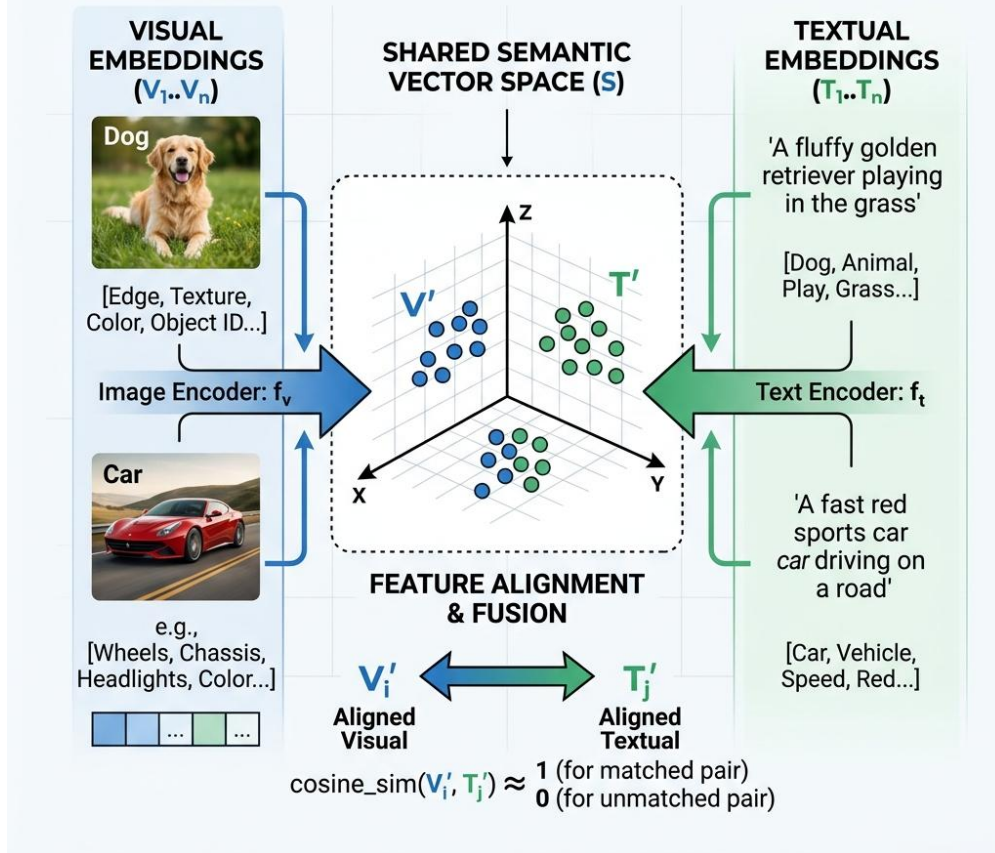
Figure 3: Conceptual alignment of visual and textual manifolds.
