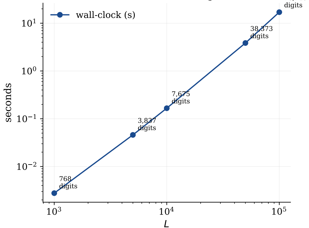
Linear snake N_L : order-12 integer recurrence
