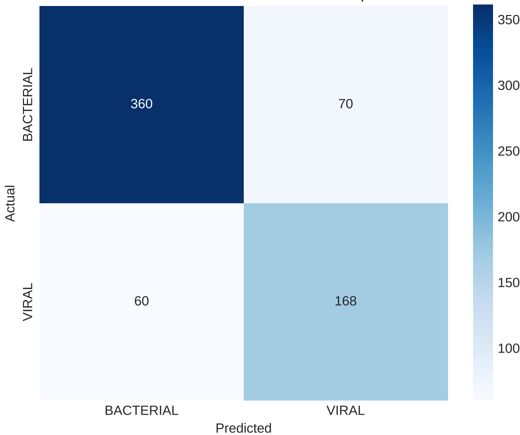
BACTERIAL vs VIRAL - DenseNet121 Patient-Safe Split Confusion Matrix
