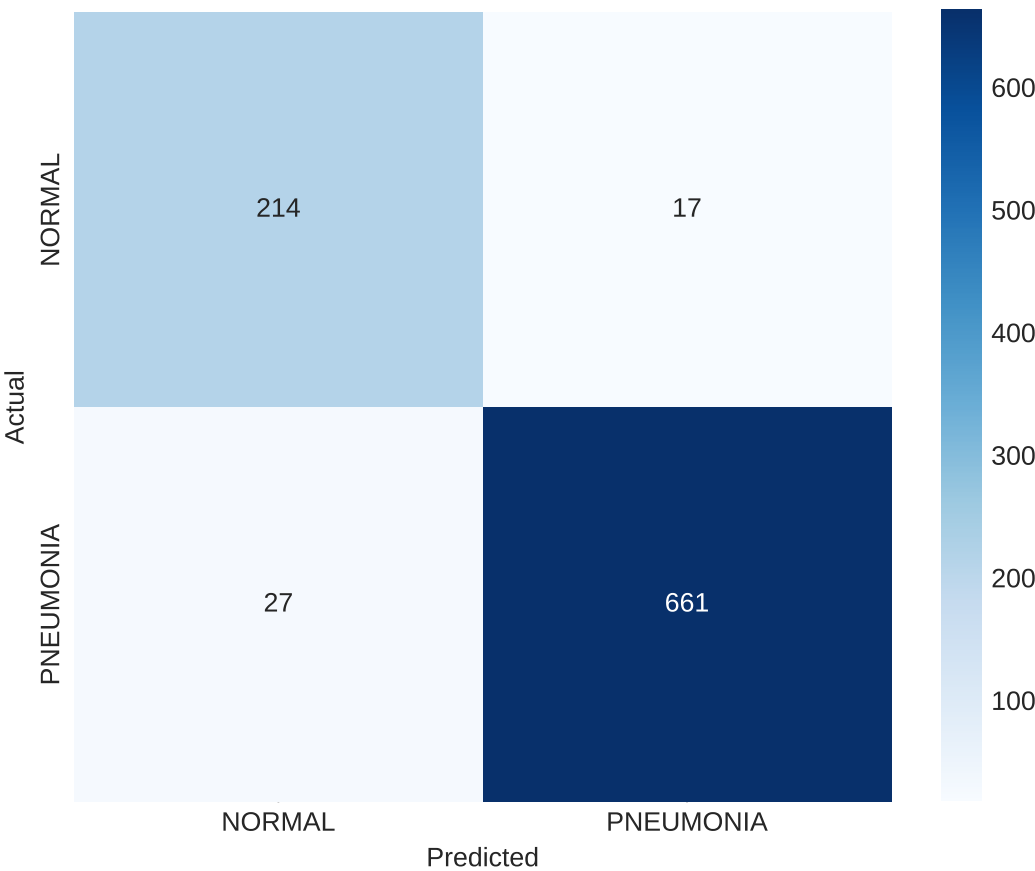
PNEUMONIA vs NORMAL - Best Saved/Current Model Confusion Matrix
