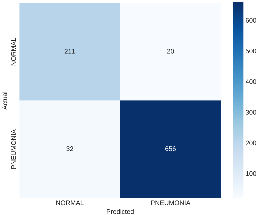
PNEUMONIA vs NORMAL Confusion Matrix
